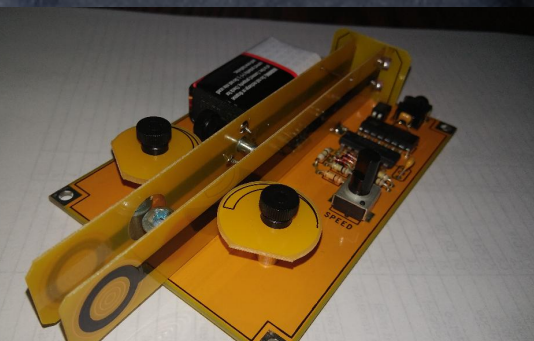
IAMBIC PADDLE WITH KEYS
